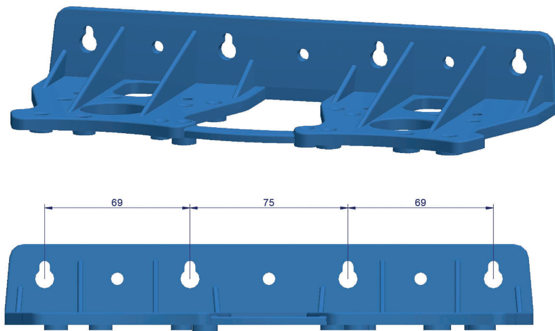
Drilling template for the mounting bracket
